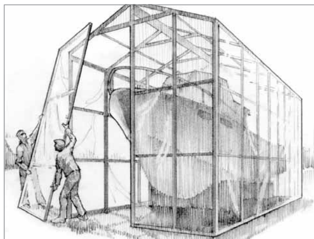
Figure 3-4 For yards repairing many boats, a drying shed built of lumber and plastic (on the order of a greenhouse) can free up valuable shop space.
